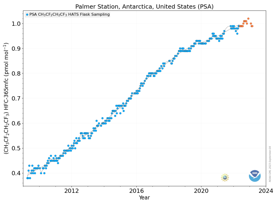
Figure 7. HFC-365mfc ( CH_3CF_2CH_2CF_3 ) levels at Palmer Station dating back to 2009, one of the Halocarbon and Trace Gases measured at Palmer Station. Orange dots are preliminary data.
