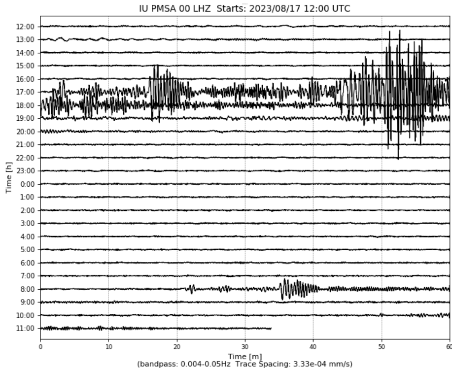
Figure 4. An August 17, 2023 earthquake near Bogota, Colombia, as recorded from the Palmer seismic station.
