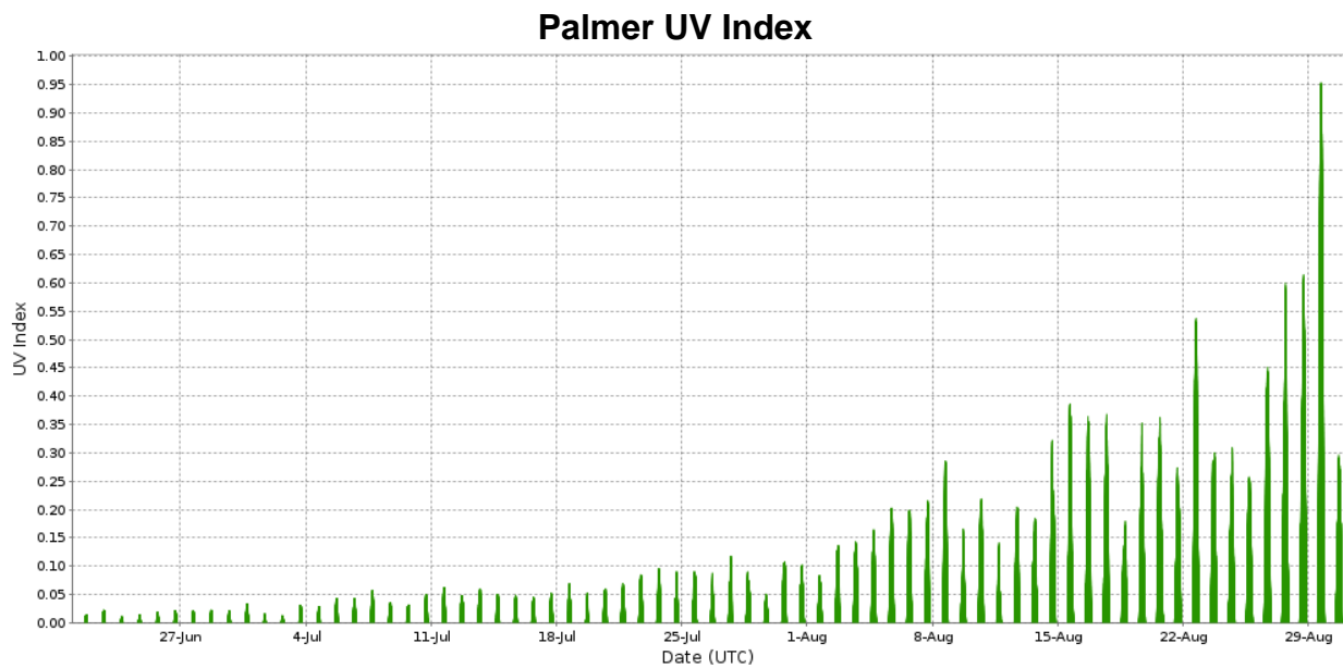
Figure 8. UV index generated from the GUV-511 radiometer, Midwinter (June 21, 2023) – August 31, 2023
